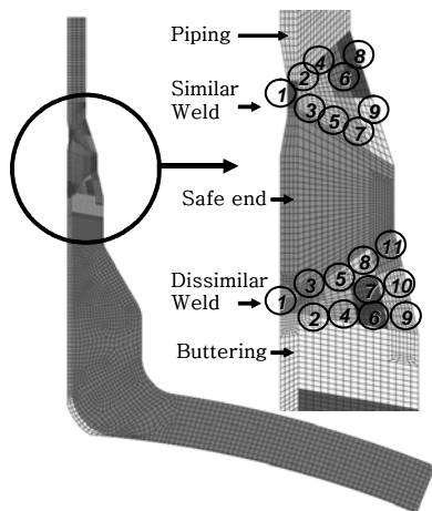
Fig. 2 Axisymmetric finite element model
