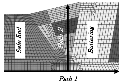
Fig. 5 Data acquisition line (path1, path2)
