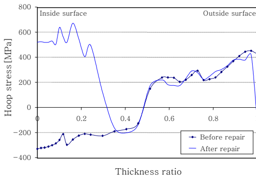
(b) Hoop stress
