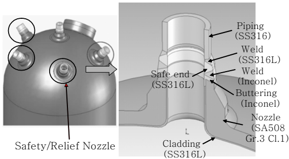
Fig. 1 PZR safety/relief nozzle(Westinghouse type)
