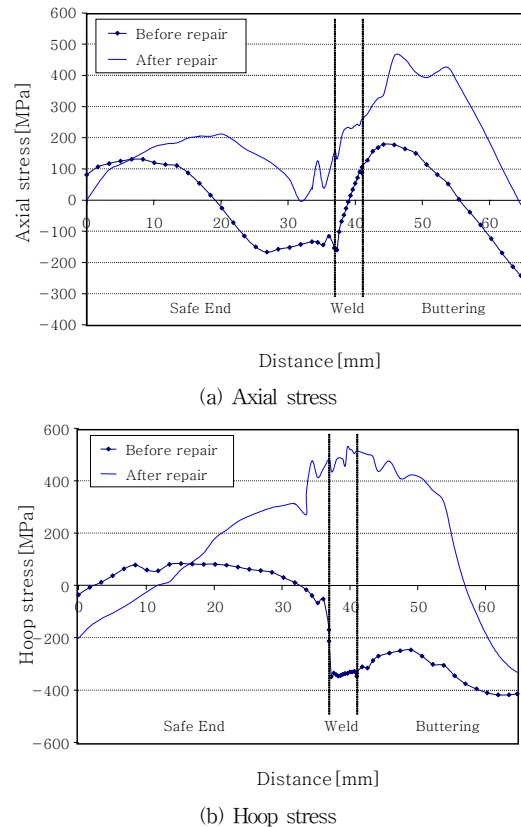
Fig. 6 Residual stress distributions after inside repair welding(path1)
