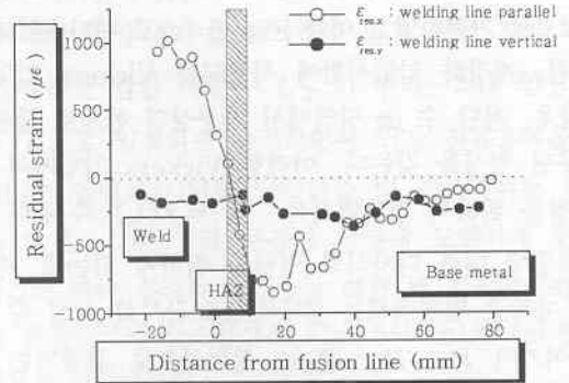
Fig. 8 Saw-cutting results(strain)
