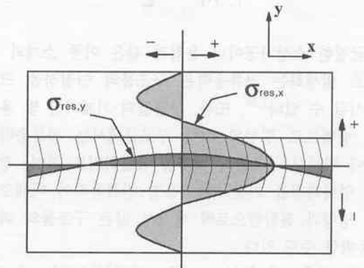
Fig. 2 General stress distribution around welded joint
