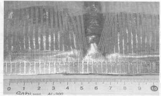
Fig. 6 Specimen used in saw-cutting test
