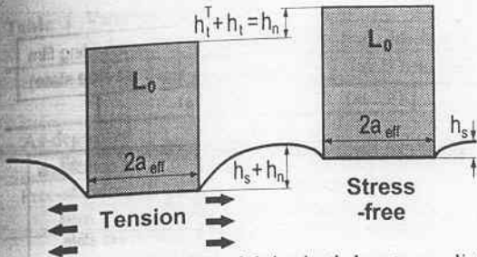
Fig. 3 Release of elastic sink-in depth by stress-relief based on the elastic flat punch theory
