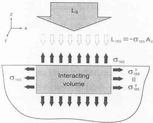
Fig. 4 Interaction of residual stress-induced normal load ( L_{res} ) and indentation load ( L_0 )
