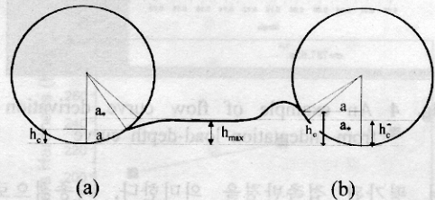
Fig. 3 The schematic diagram of indentation (a) sink-in and (b) pile-up phenomena
